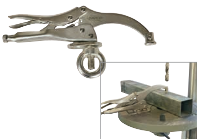
9" DRILL PRESS LOCKING CLAMP • 2" (50mm) max. jaw opening • 3" (75mm) throat depth • Fastens to drill press slot • Secures work pieces tightly
